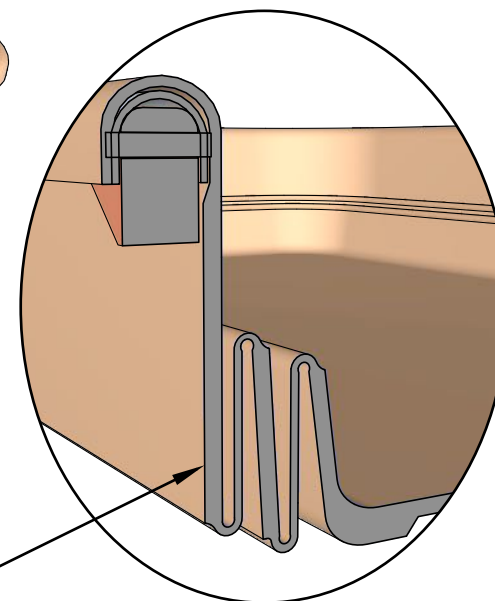
Folding section close-up
